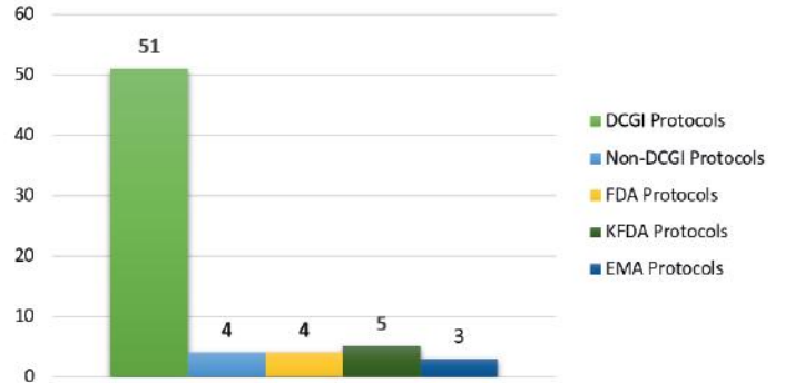
Protocol Statistics
